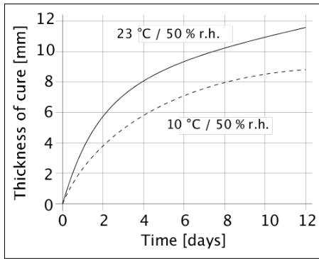
Diagram 1: Curing speed SikaTack® Go4it!
